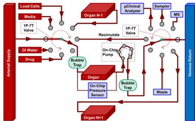
Fig. 5. Conceptual drawing of how two single-pole, seven-throw (1P-7 T) valves and an on-chip peristaltic pump could provide the requisite PC functions in Fig. 2. The valve configuration shown has perfusate from the arterial supply perfusing Organ N and then exiting into the venous return. Other configurations of the valve on the left are used for adding media to make up any that is removed for sampling or flushing, loading cells (with the effluent going to waste), accepting fluid from an upstream organ, local recirculation, infusing a drug, dye, or marker into the single organ, or adding deionized (DI) water to adjust osmolarity after evaporation of water out of the device. The valve on the right is for venous return (as configured), sending fluid to a downstream organ, waste, recirculations, the \mu\text{CA} , an external autosampler, or an online MS. A second PC might be required to prepare cells in any secondary spaces, for example, to establish a confluent alveolar epithelium in a lung.
