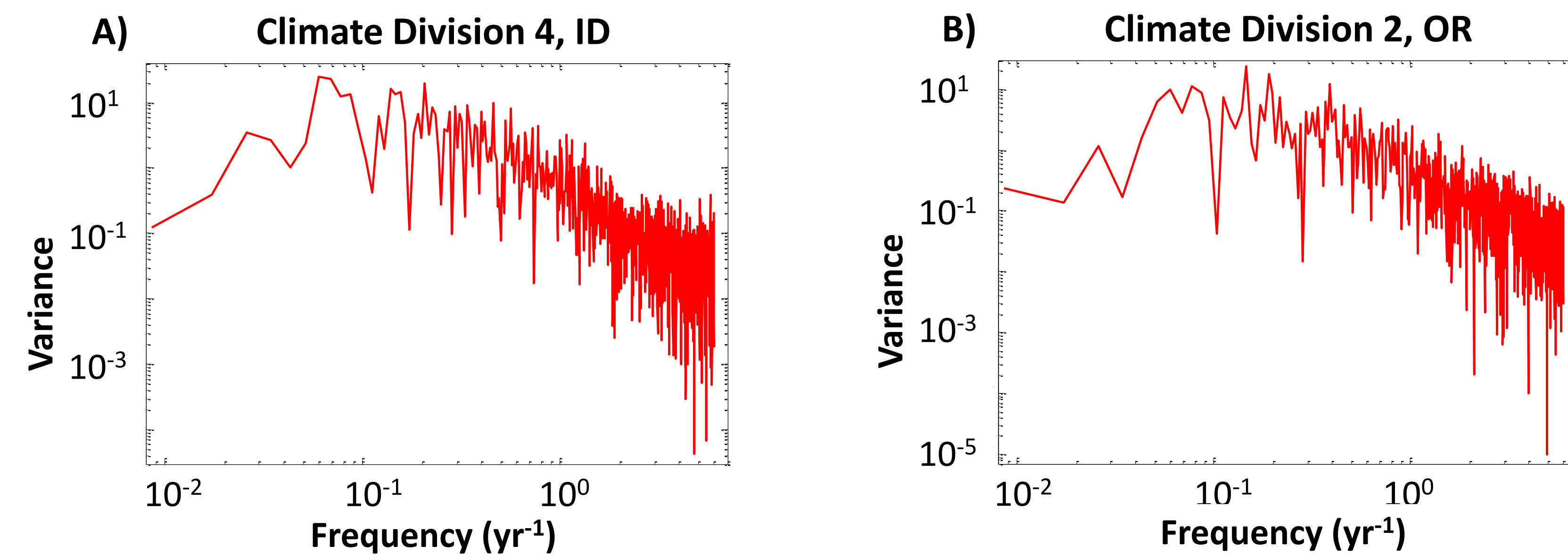
Figure 2: Continuous periodogram of filtered monthly PDSI data for A) Climate Division 4 of Idaho, and B) Climate Division 2 of Oregon. Data was filtered using a cutoff frequency of 1/70.
