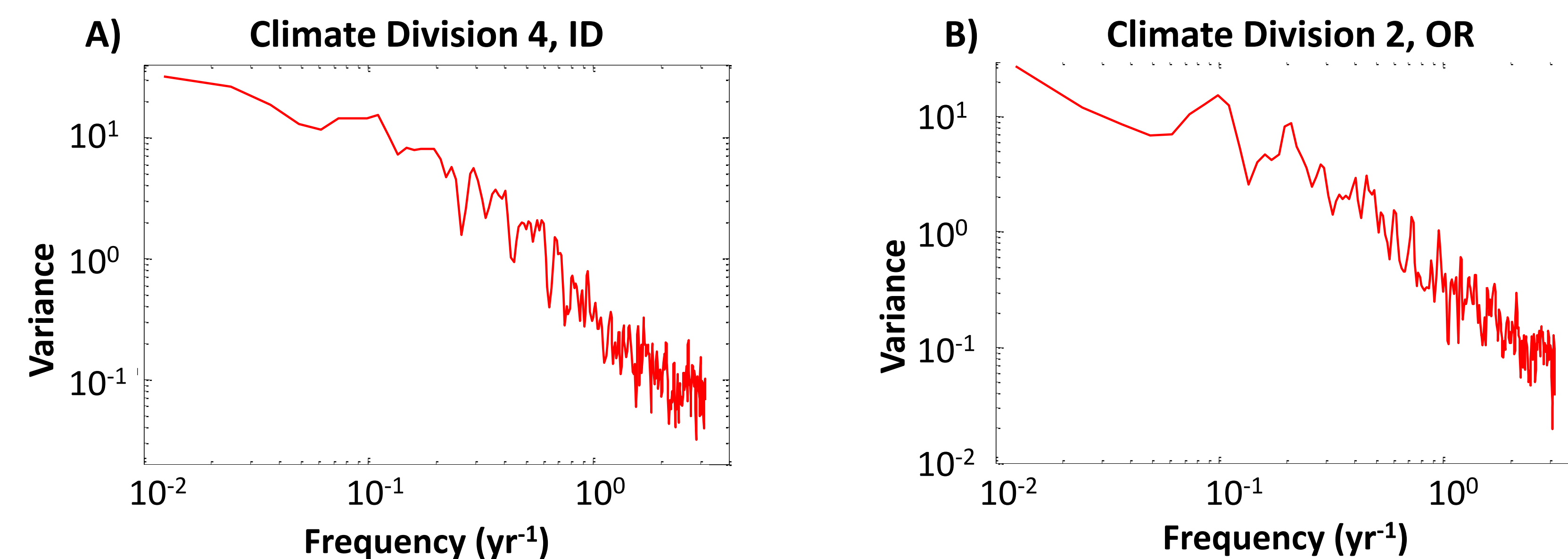
Figure 3: Power spectral density of monthly PDSI data for A) Climate Division 4 of Idaho, and B) Climate Division 2 of Oregon. The power spectral densities were calculated using Welch's method.
