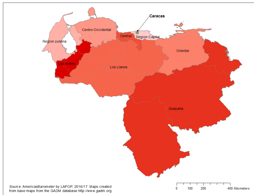
Figure 1: Sample stratification in Venezuela
