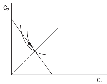
Figure 1.15 \rho > r
