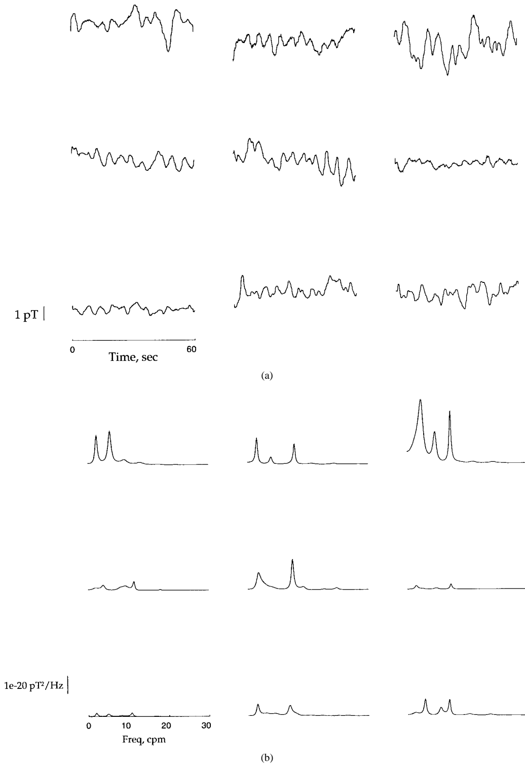
Fig. 5. Small bowel signals. (a) The small bowel projections of the magnetic field recorded at all nine abdominal locations are shown for a typical subject. Slow waves characteristic of intestinal activity are evident. (b) The AR power spectra corresponding to the signals in (a). Peaks in the 8–12 cpm range indicate small intestinal activity. Some sections exhibit multiple peaks indicating different GI sources.
