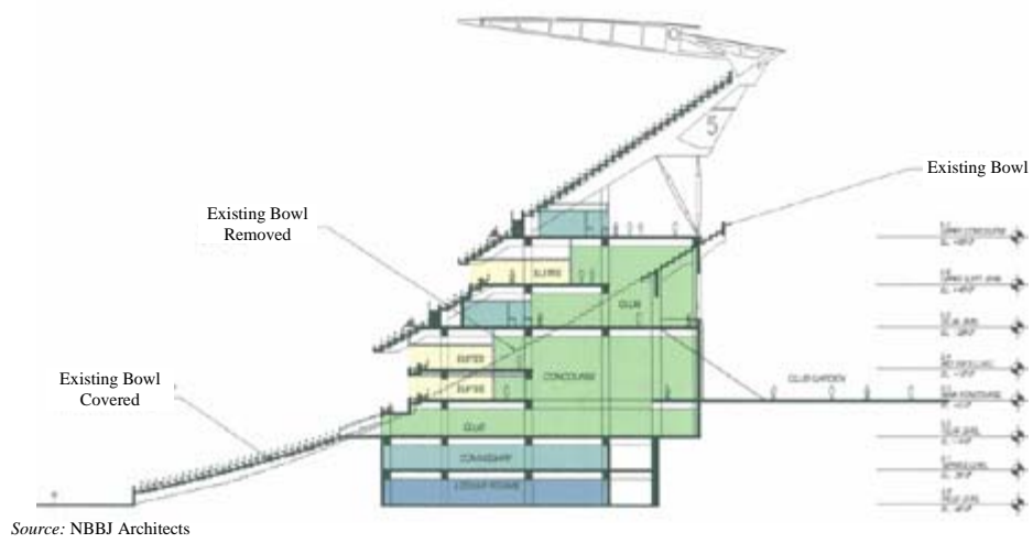
Figure 1. L. A. Coliseum Proposed Renovations
