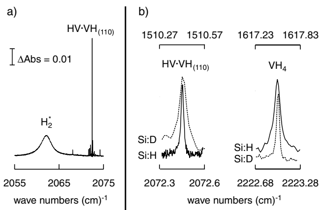
FIG. 1. (a) Section of the IR absorbance spectrum of e^- -irradiated, H-doped Si, showing the lines of HV \cdot VH_{(110)} and H_2^* . (b) Comparison of the Si-H (full) and Si-D (dashed) absorption lines of HV \cdot VH_{(110)} and VH_4 . The instrumental resolution was 0.025 \text{ cm}^{-1} , except for the 2072.5\text{-cm}^{-1} line which was measured with a resolution of 0.006 \text{ cm}^{-1} .
